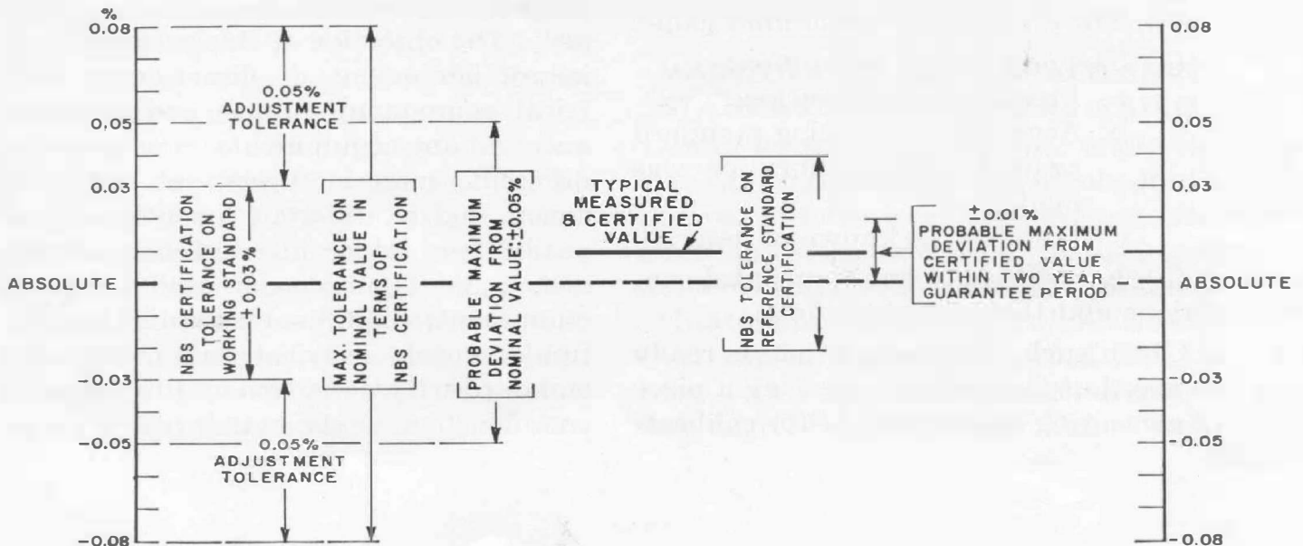
Figure 3. Chart showing the relation between nominal and calibrated values for a General Radio standard of capacitance or inductance.
