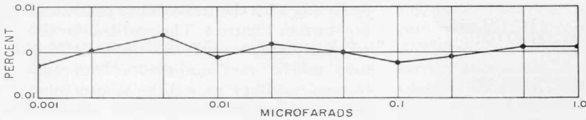
Figure 5. Plot showing consistency between General Radio-derived values and NBS calibration of General Radio reference standards after adjustment for over-all level.
