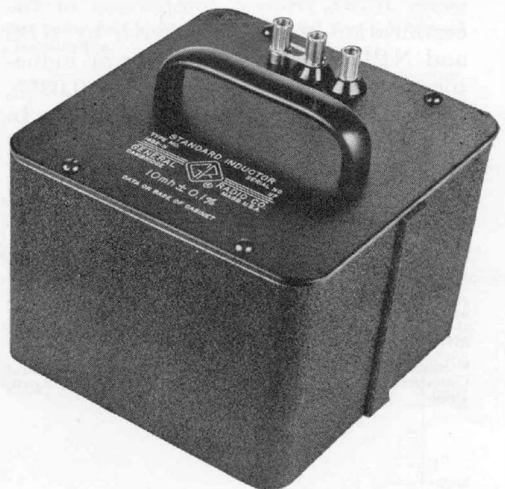
Figure 1. A stable low-frequency inductance standard, the General Radio Type 1482 Standard Inductor.
